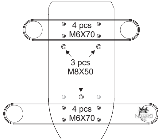
Bottom view Tweeter/Mid Tower
