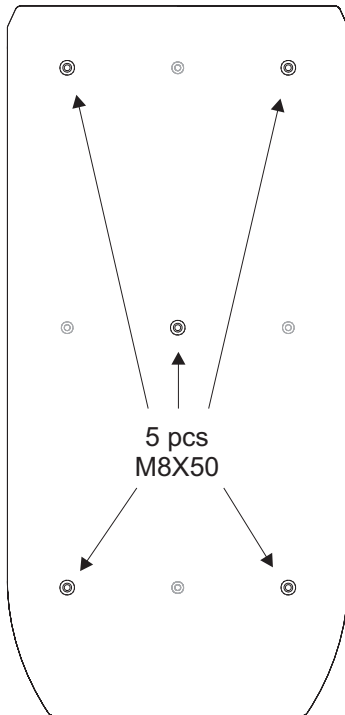
Top view Bass Tower
