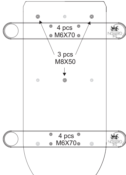
Bottom view Bass Tower
